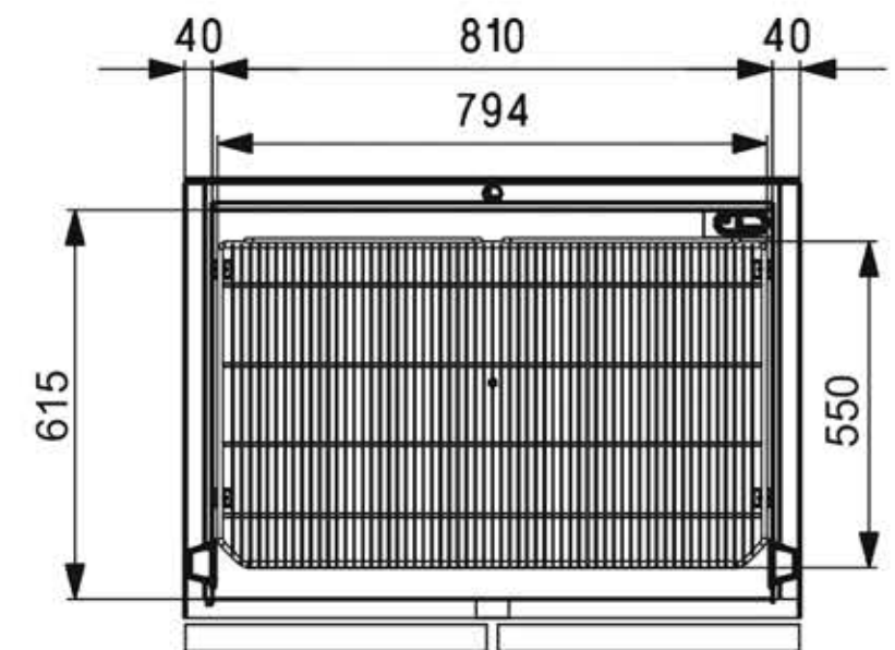
SECTION B-B
